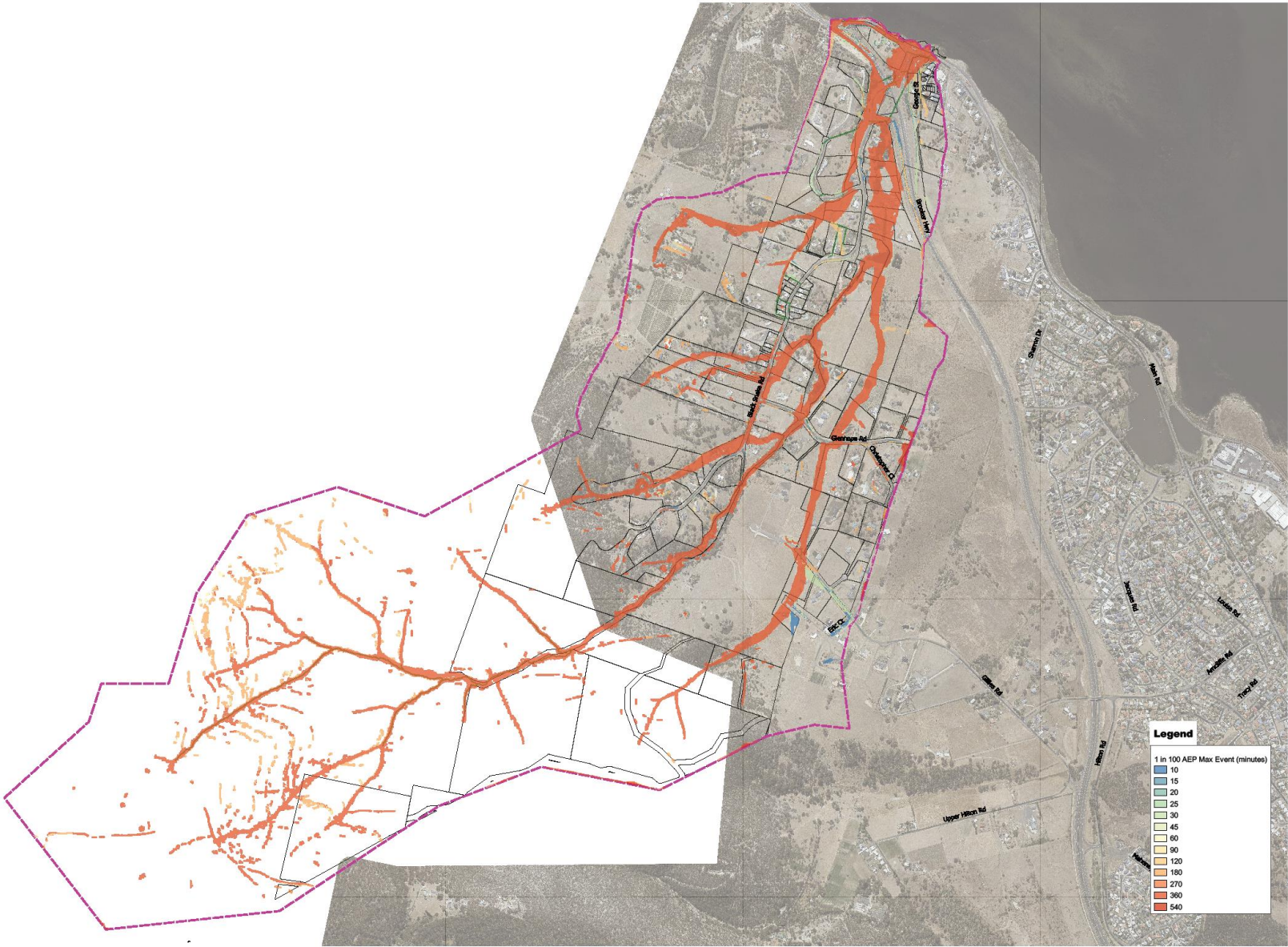
Figure Title : 1 in 100 AEP Critical Duration Coordinate System : Universal Transverse Mercator Projection, MGA Zone 55 South, Geodetic Datum of Australia (GDA95) Page Size : A1 Scale : 1:6,800 Project Title : Glenorchy Municipality - Black Snake Rivulet SSMP
